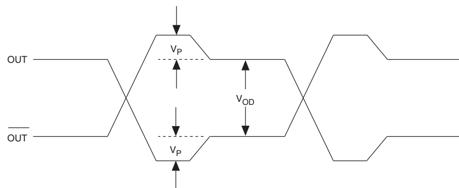
Figure 8-9. Programmable Pre-Emphasis (1)
