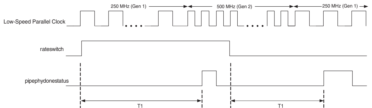
Figure 1-91. Rateswitch in PCIe Mode (1)
