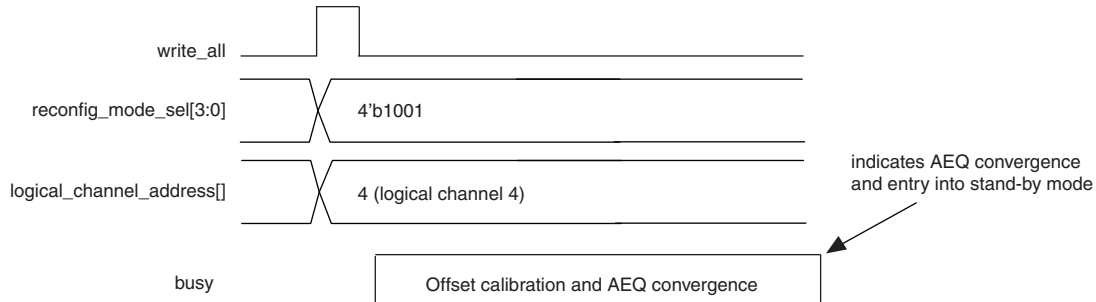
Figure 5-39. AEQ Timing Diagram in One-Time Adaptation Mode
