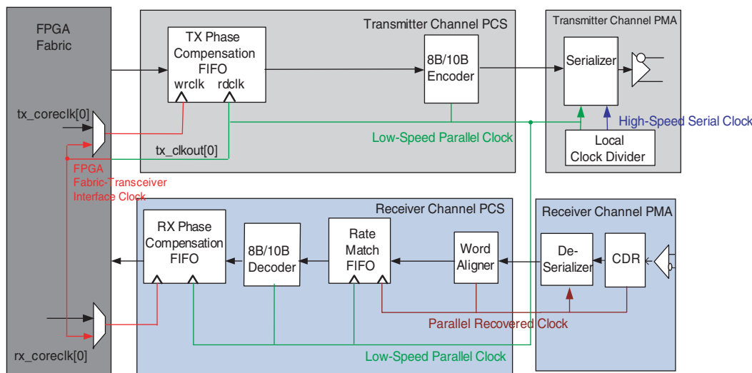
Figure 1-133. GIGE Mode Datapath
