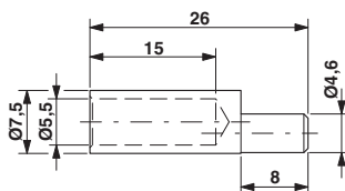
Dimensional drawing
