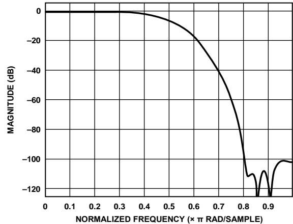
Figure 69. HB2 Filter Response
